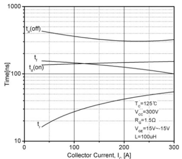
Fig 6. Typical Switching Time vs. Collector Current
